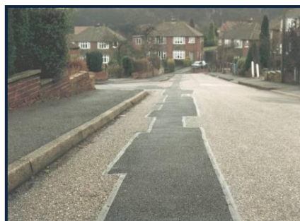
Overbanding of reinstatement in N Derbyshire Housing Estate Client Severn Trent Water
