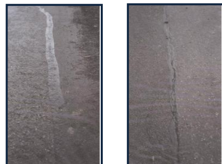
Viatec Overbanding Tape (L) Hot Poured Bitumen (R) Comparison, both applied on same date at road junction.
